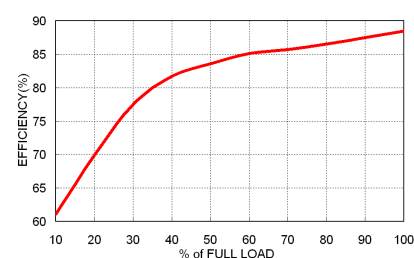
FKC12-48S05W Efficiency vs. Output Load
