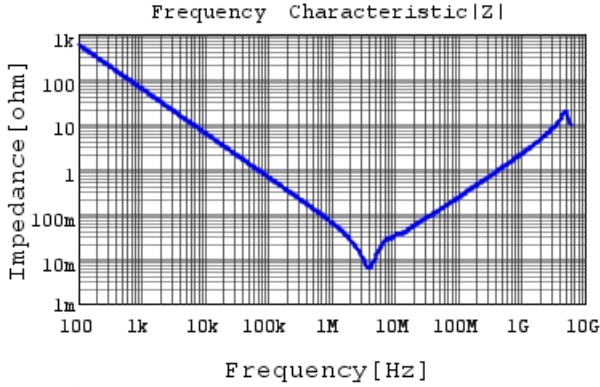
GRM21BR71C475KA73 |Z| DCOV, 25degC
