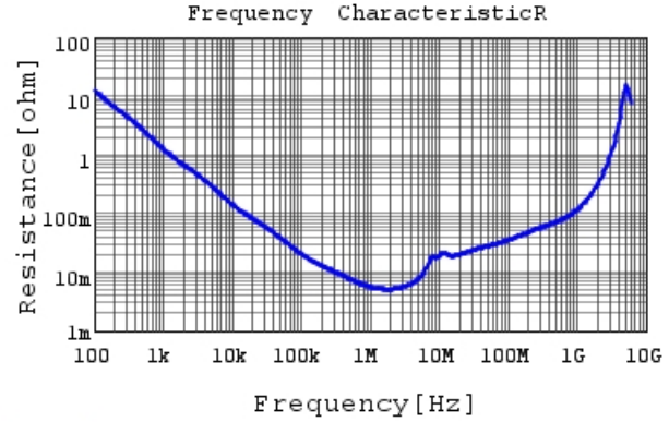
GRM21BR71C475KA73 R DCOV, 25degC
