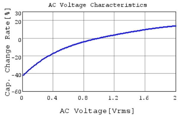
GRM21BR71C475KA73 C-AC Voltage capchange, DC
