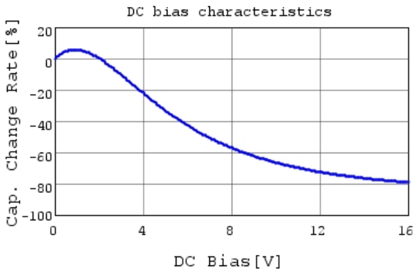
GRM21BR71C475KA73 C-DC bias capchange, 25.0c
