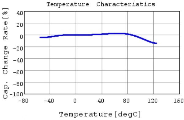
GRM21BR71C475KA73 C-Temp. capchange, DC0.0V,
