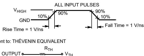
Figure 6. AC Test Loads and Waveforms
