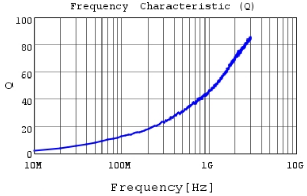
LQP03TN0N9C02 Q
