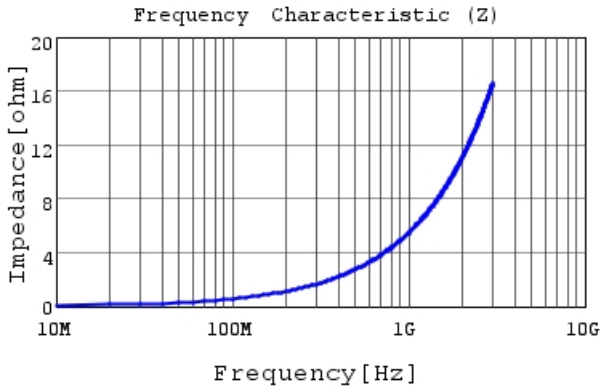
LQP03TN0N9C02 |Z|
