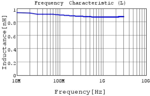
LQP03TN0N9C02 L
