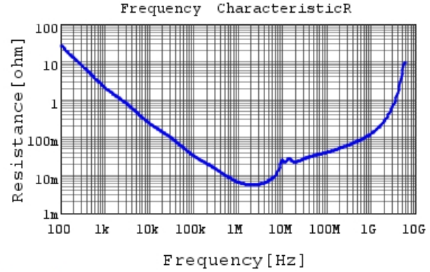
GRM21BR71E225KA73 R DCOV, 25degC
