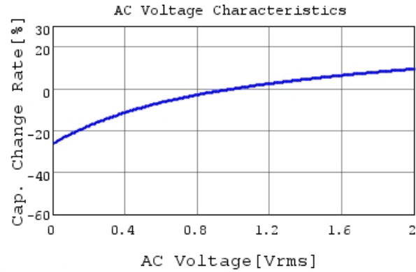
GRM21BR71E225KA73 C-AC Voltage capchange, Dc
