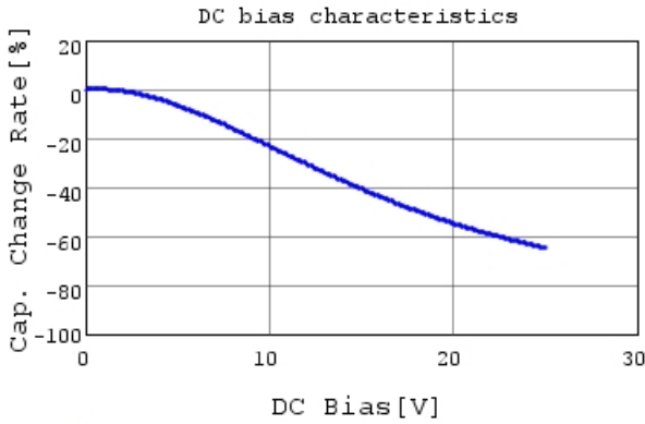
GRM21BR71E225KA73 C-DC bias capchange, 25.0c
