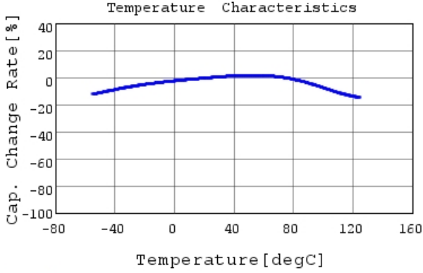
GRM21BR71E225KA73 C-Temp. capchange, DC0.0V,
