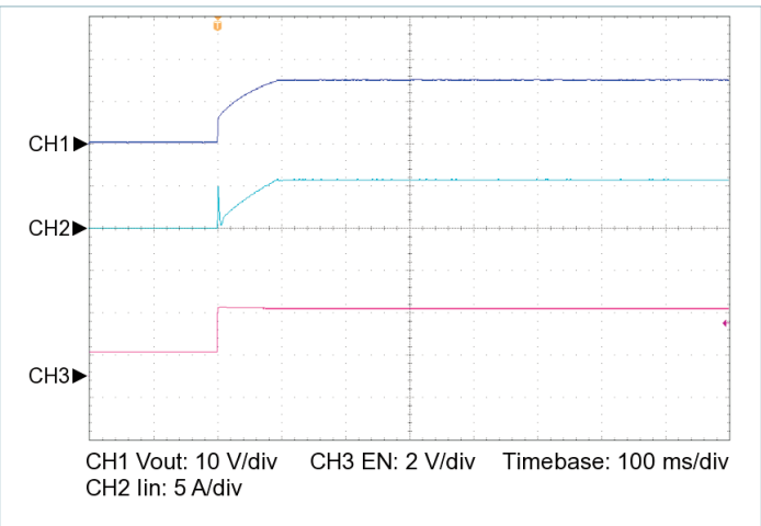
Figure 14 — Startup from EN, V_{IN} = 30\text{ V} , C_{OUT\_EXT} = 10000\text{ }\mu\text{F} , R_{LOAD} = 1.402\text{ }\Omega
