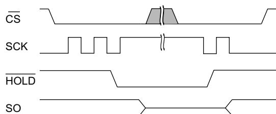
Figure 27. HOLD Operation
