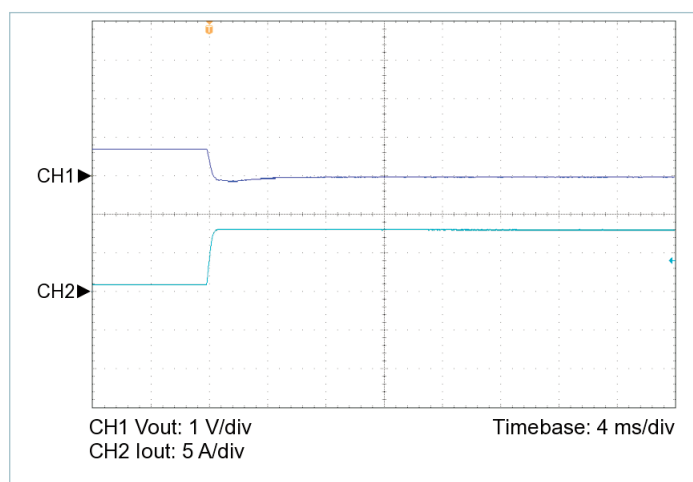
Figure 20 — 10% to 100% load transient response, V_{IN} = 100\text{ V} , nominal trim, C_{OUT\_EXT} = 470\text{ }\mu\text{F}
