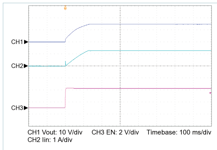
Figure 16 — Startup from EN, V_{IN} = 100\text{ V} , C_{OUT\_EXT} = 10000\text{ }\mu\text{F} , R_{LOAD} = 1.875\text{ }\Omega
