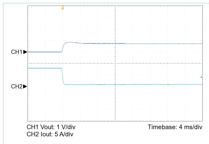
Figure 19 — 100% to 10% load transient response, V_{IN} = 100\text{ V} , nominal trim, C_{OUT\_EXT} = 470\text{ }\mu\text{F}
