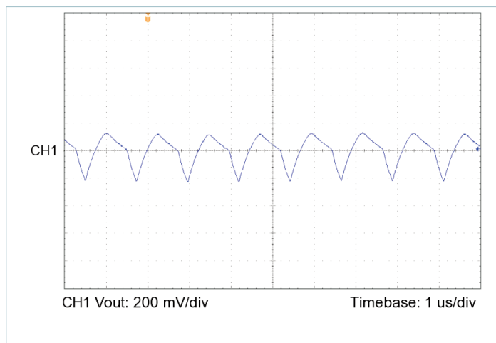
Figure 15 — Output voltage ripple, V_{IN} = 100\text{ V} , V_{OUT} = 15.0\text{ V} , C_{OUT\_EXT} = 470\text{ }\mu\text{F} , R_{LOAD} = 1.875\text{ }\Omega
