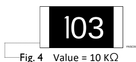
Fig. 4 Value = 10 K \Omega
