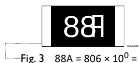
Fig. 3 88A = 806 \times 10^0 = 806 \Omega
