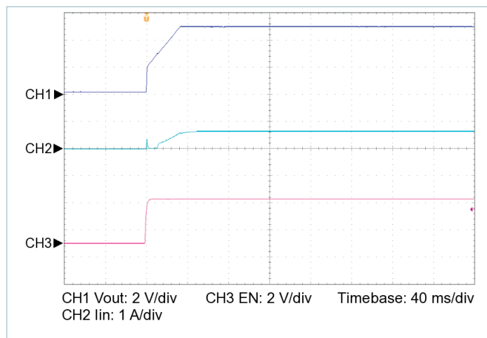
Figure 16 — Startup from EN, V_{IN} = 100\text{ V} , C_{OUT\_EXT} = 10000\text{ }\mu\text{F} , R_{LOAD} = 0.417\text{ }\Omega
