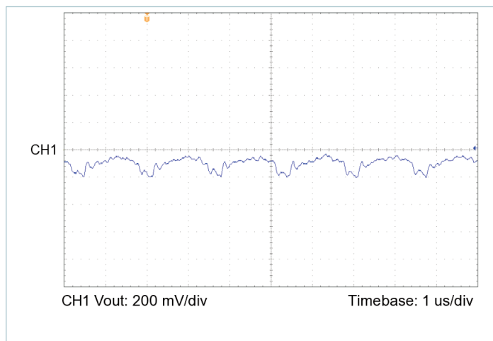
Figure 15 — Output voltage ripple, V_{IN} = 100\text{ V} , V_{OUT} = 5.0\text{ V} , C_{OUT\_EXT} = 470\text{ }\mu\text{F} , R_{LOAD} = 0.417\text{ }\Omega
