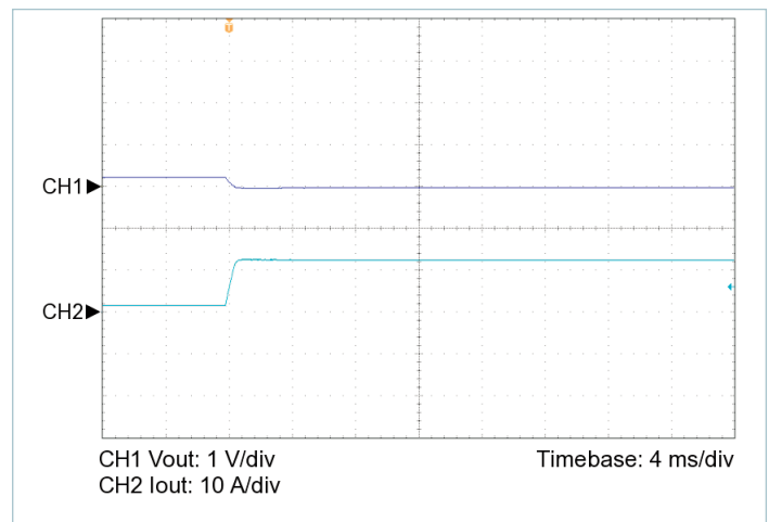
Figure 20 — 10% to 100% load transient response, V_{IN} = 100\text{ V} , nominal trim, C_{OUT\_EXT} = 470\text{ }\mu\text{F}
