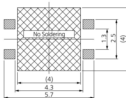
Land pattern
