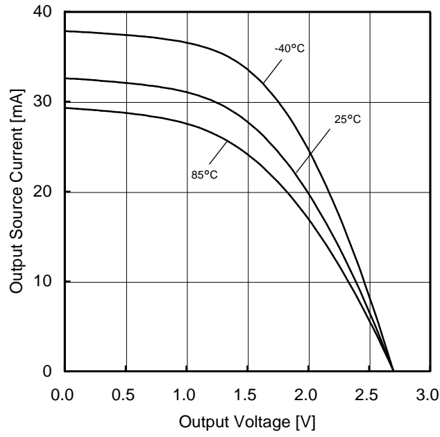
Figure 32. Output Source Current vs Output Voltage ( V_{DD}=2.7V )
