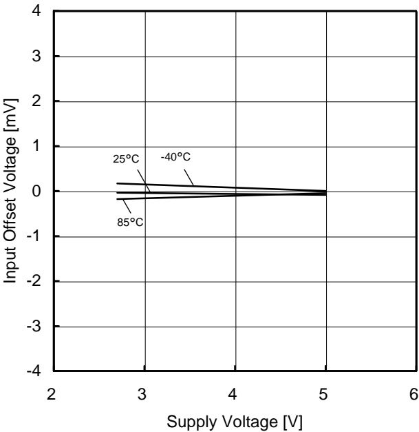
Figure 58. Input Offset Voltage vs Supply Voltage ( V_{ICM}=VDD/2 , E_K=-VDD/2 )
