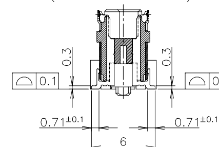
SECT. Y-Y (GROUND POSITION)
