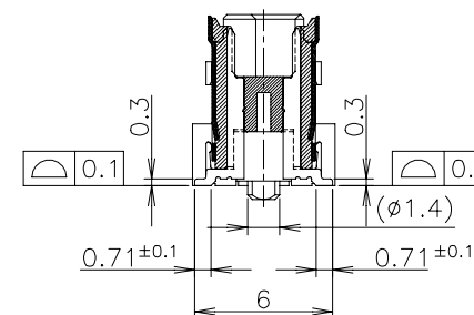
SECT. Z-Z (SIGNAL POSITION)
