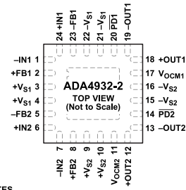
Figure 5. ADA4932-2 Pin Configuration
