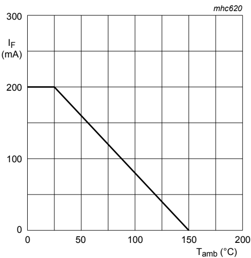
Fig. 5. Forward current as a function of ambient temperature; derating curve
