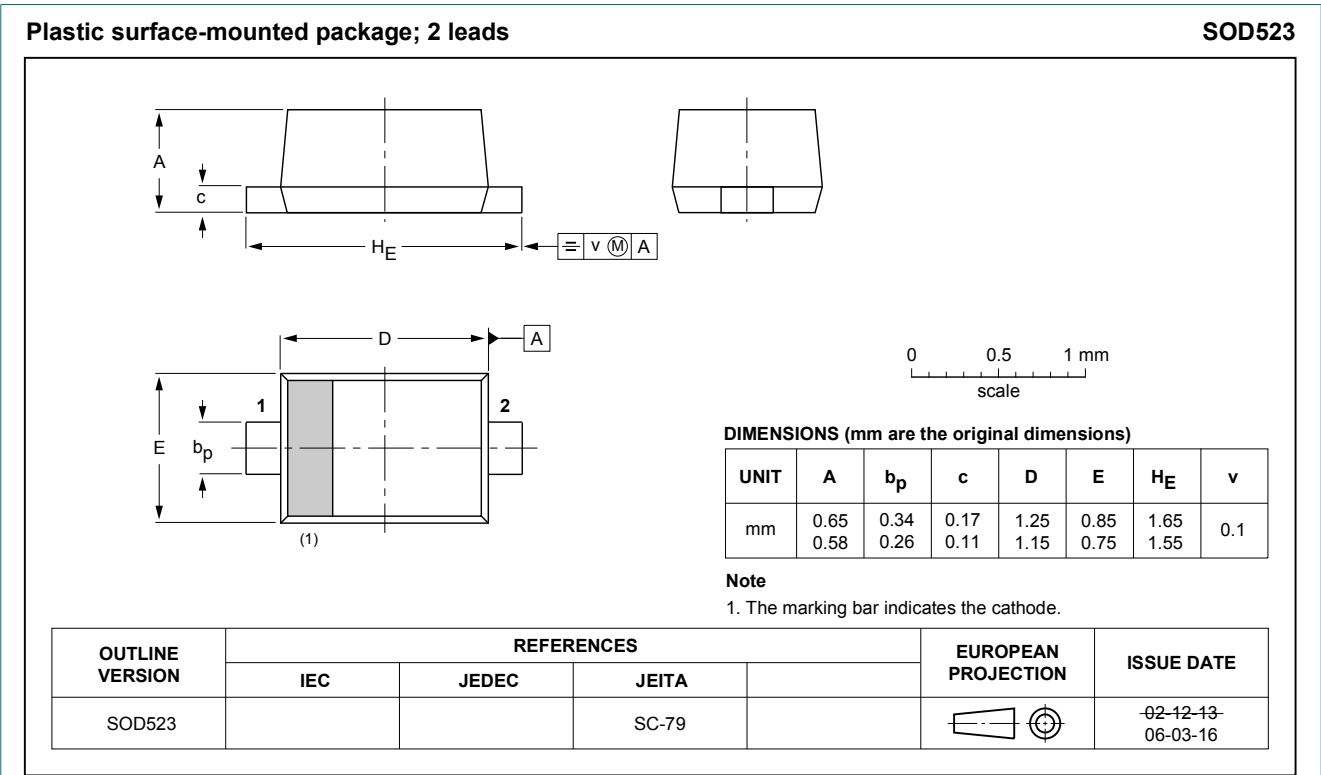
Fig. 9. Package outline SOD523
