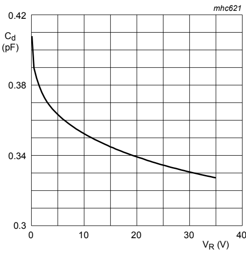
Fig. 6. Diode capacitance as a function of reverse voltage; typical values f = 1\text{ MHz} T_{amb} = 25\text{ °C}
