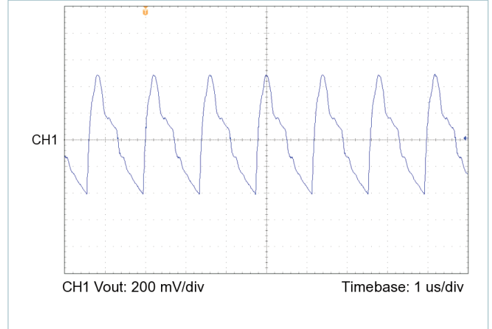
Figure 16 — Output voltage ripple, V_{IN} = 28\text{ V} , V_{OUT} = 48.0\text{ V} , C_{OUT\_EXT} = 200\text{ }\mu\text{F} , R_{LOAD} = 7.200\text{ }\Omega
