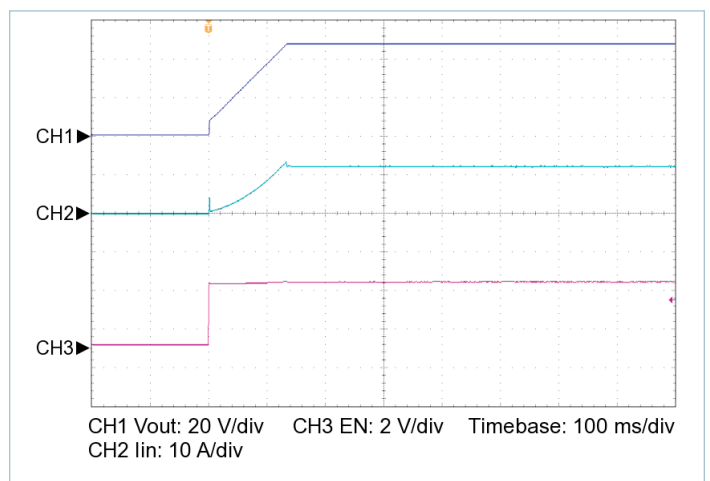
Figure 14 — Startup from EN, V_{IN} = 28\text{ V} , C_{OUT\_EXT} = 2000\text{ }\mu\text{F} , R_{LOAD} = 7.200\text{ }\Omega
