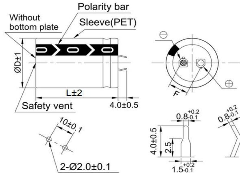
(PC board hole dimensions) (Terminal dimensions)
