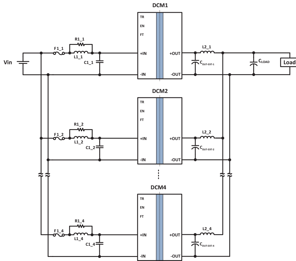
Typical Application 1: DCM4623xD2H15E0yzz in an array of four units
