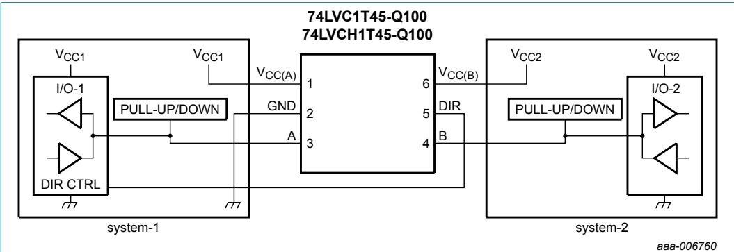
Fig. 15. Bidirectional logic level-shifting application
