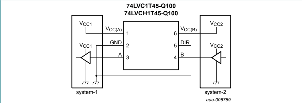
Fig. 14. Unidirectional logic level-shifting application
