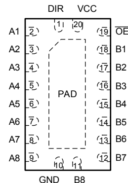
Figure 5-2. SN74AHC245-Q1 WRKS Package, 20-Pin WQFN (Top View)
